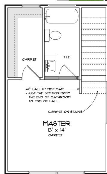
3RD FLOOR
