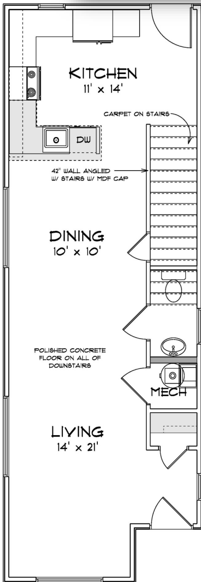
MAIN FLOOR
