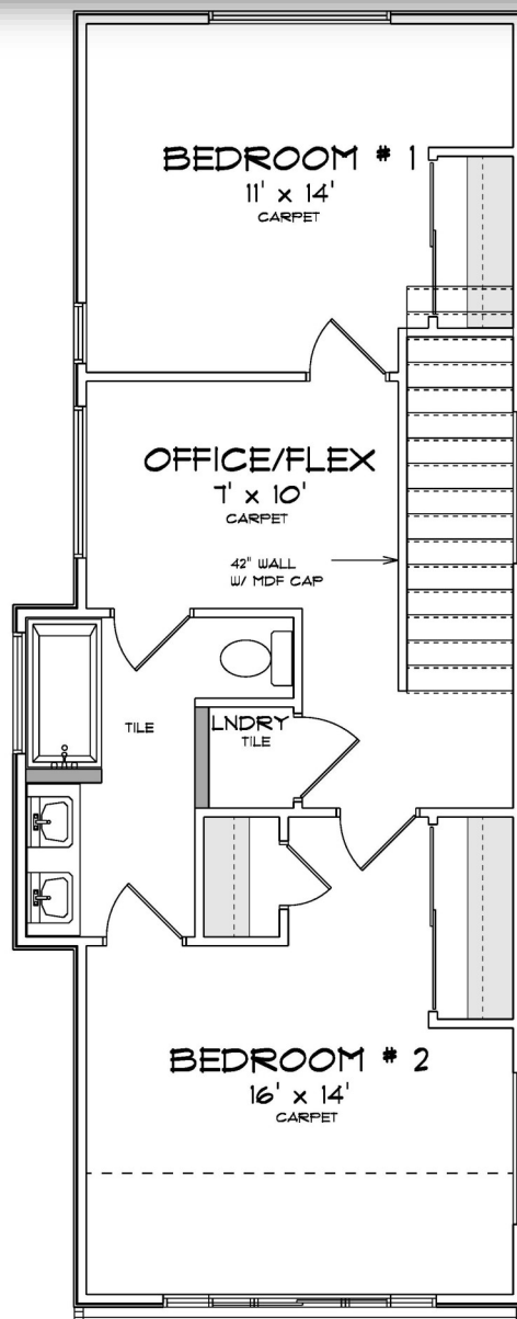
2ND FLOOR
